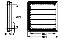
LOUVRE SHUTTER
